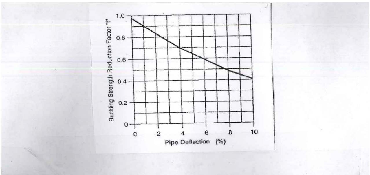
Figure 2 – Reduction Factor for Buckling Strength (I) Due to Deflection in Round Pipe
