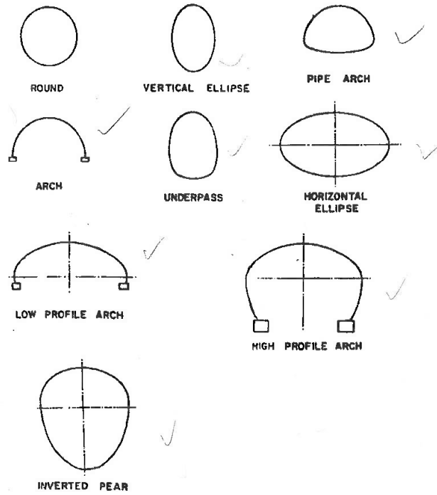
FIGURE 12.7.1A Standard Terminology of Structural Plate Shapes Including Long-Span Structures
