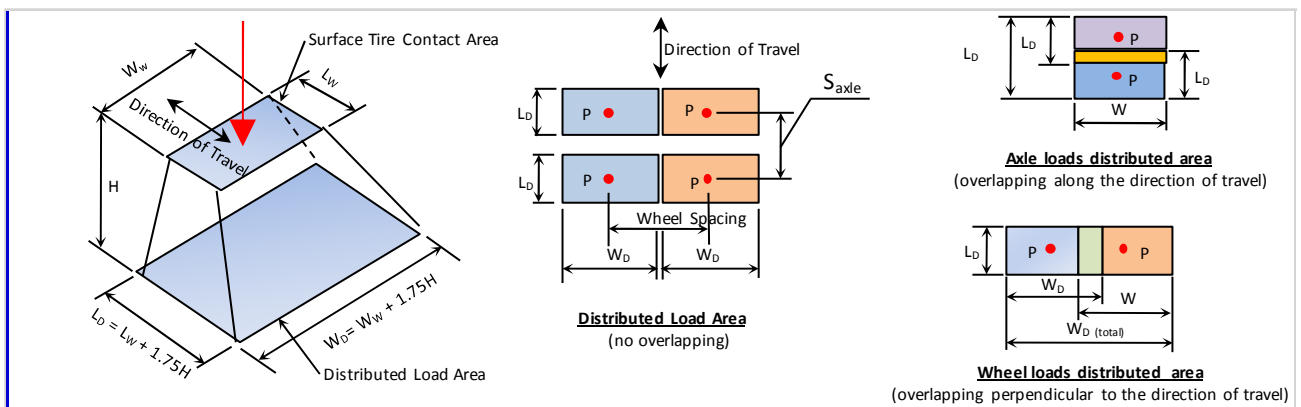
Figure 3 – Distributed Load Area for Single and Overlapped Loads
