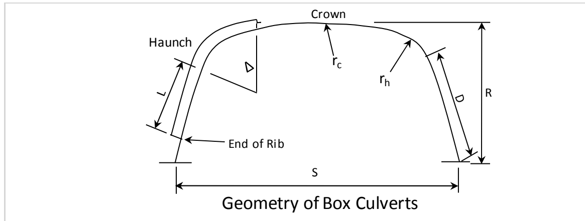
Figure 4 – Structural Plate Box Culverts
