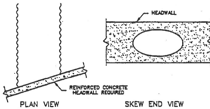
(C) SKEW CUT END (REQUIRES FULL HEADWALL)
