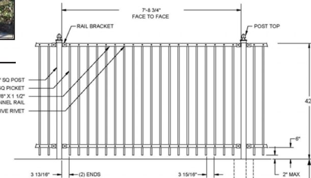
IMPERIAL FENCE 'A'
