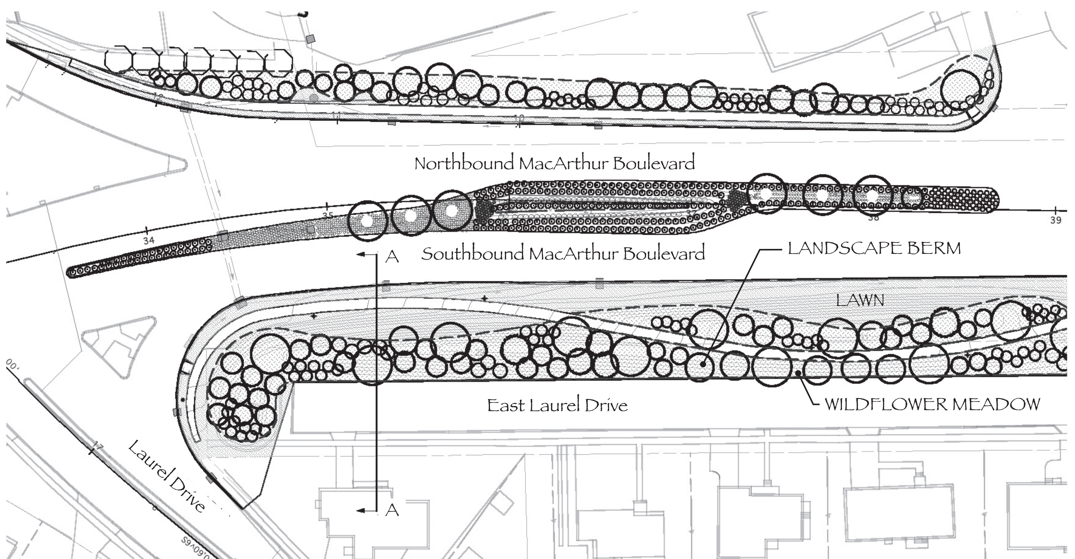
LANDSCAPE BERM PLAN
