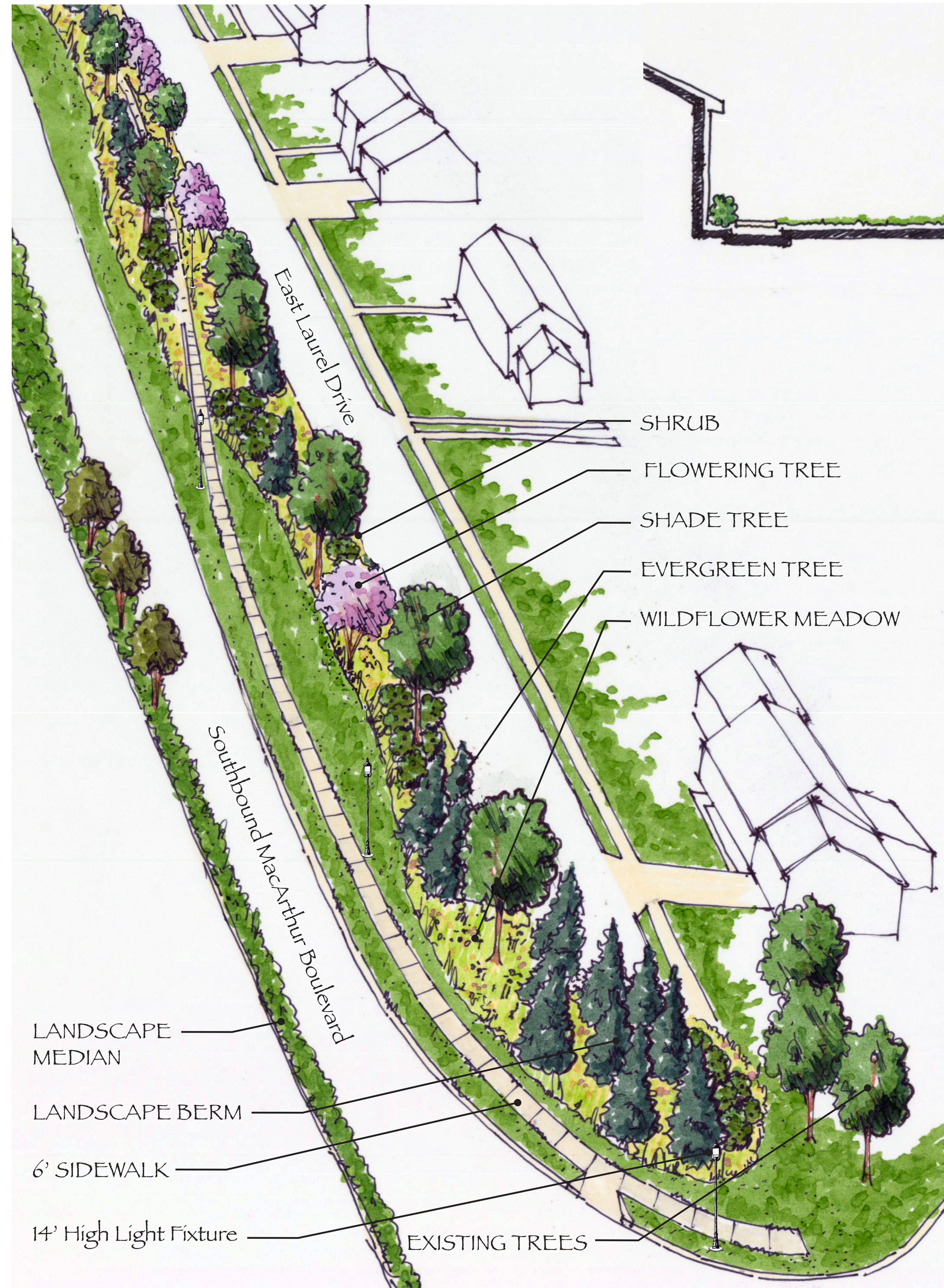
LANDSCAPE BERM PERSPECTIVE
