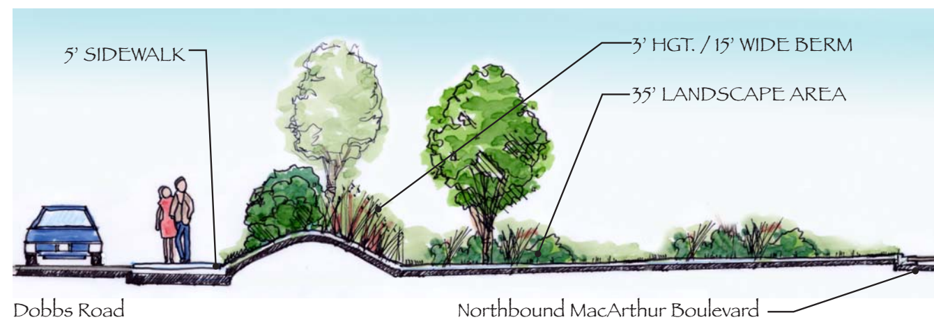
LANDSCAPE BERM SECTION B-B'
